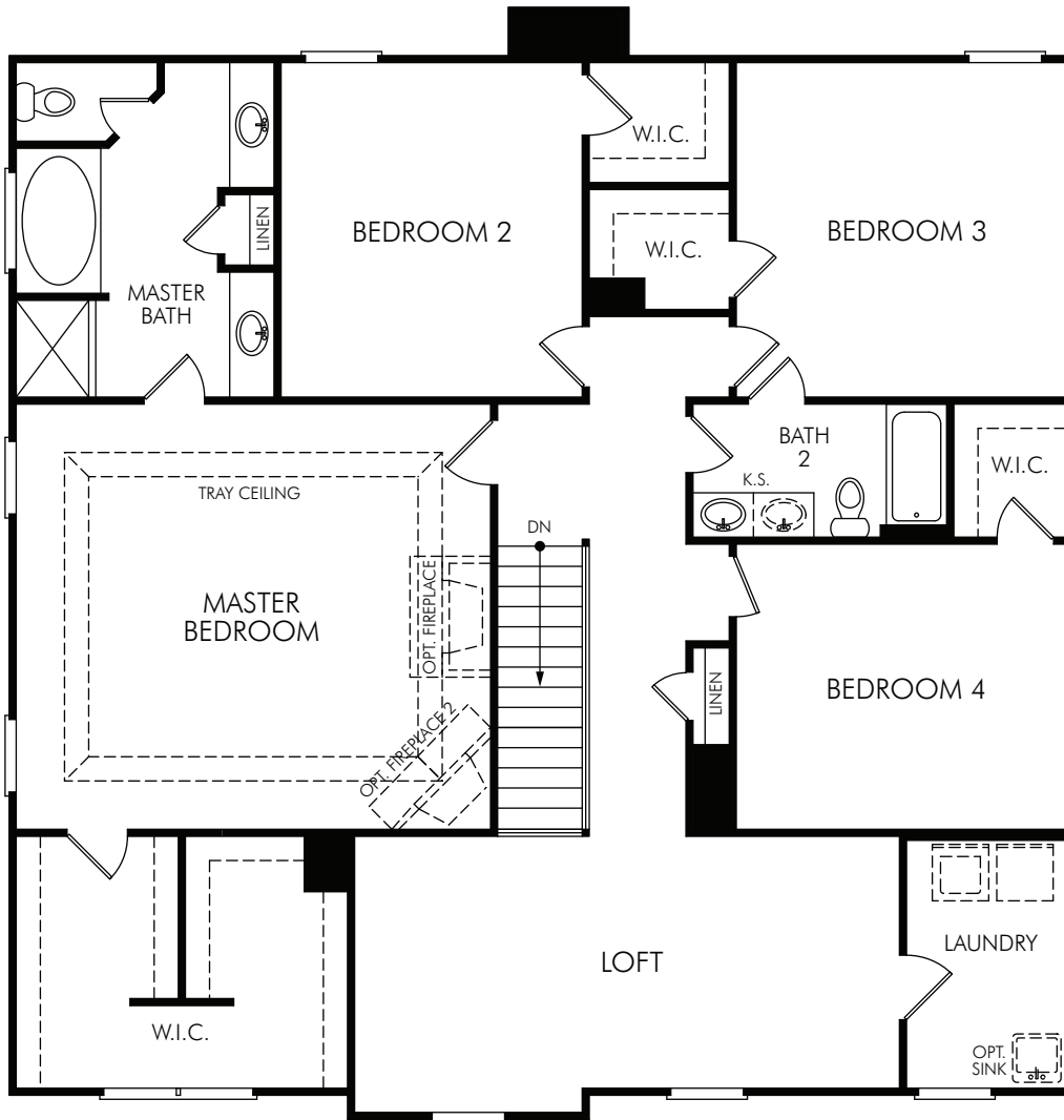
SECOND FLOOR PLAN LOFT OPTION 2-A
