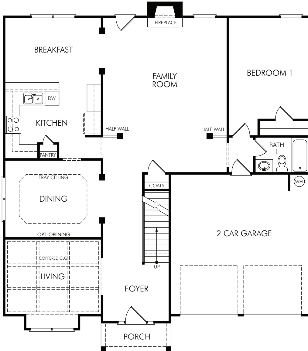
FIRST FLOOR
