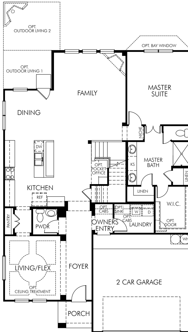
FIRST FLOOR
