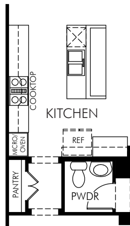
OPT. KITCHEN
