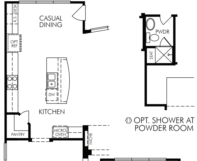
⑦ OPT. KITCHEN 1
