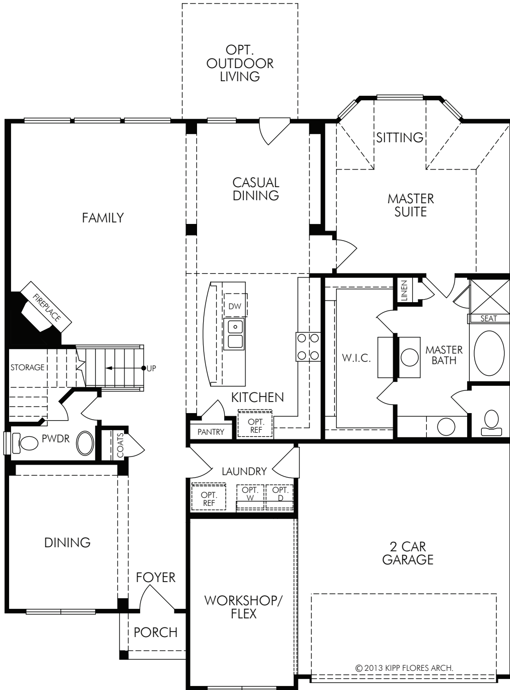
FIRST FLOOR
