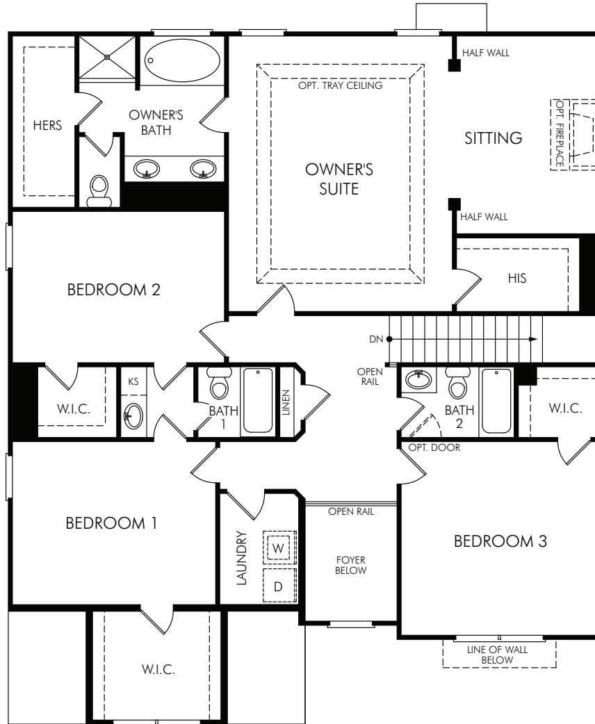
OPT. SECOND FLOOR 2-A
