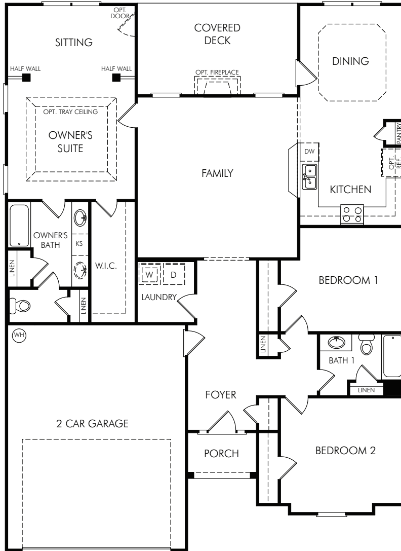
FIRST FLOOR PLAN - SLAB
