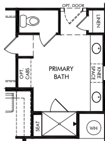
OPT. EXPANDED PRIMARY SHOWER
