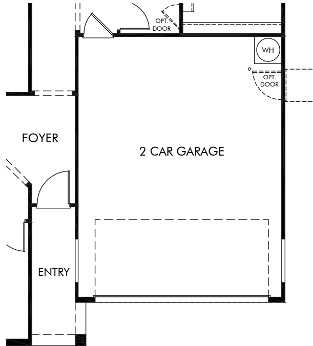
OPT. 4' GARAGE EXTENSION
