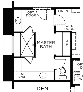
OPT. EXPANDED SHOWER AT MASTER BATH
