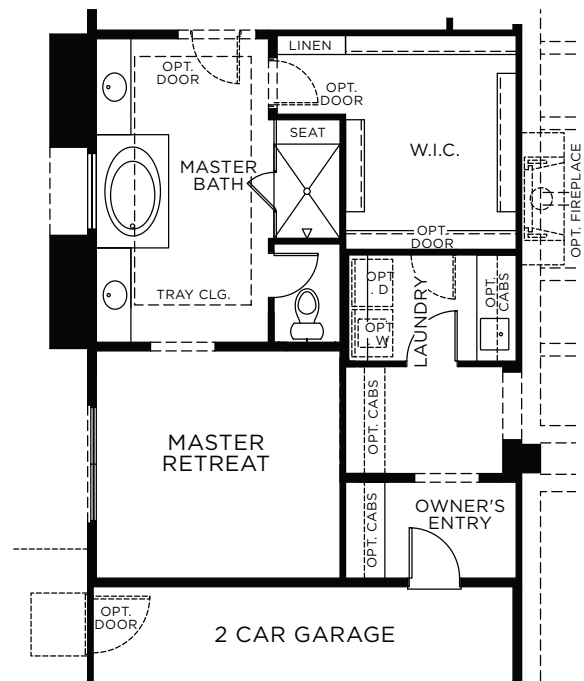
OPT. MASTER RETREAT ILO DEN
