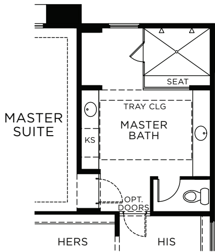
OPT. EXPANDED SHOWER AT MASTER BATH
