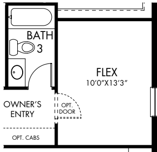
OPT. FLEX ILO BEDROOM 4
