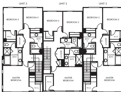
THIRD FLOOR
