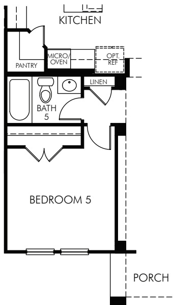
⑭ OPT. BEDROOM 5 / BATH 5 w/ OPT. KITCHEN BTH0505/ KIT1000 WINDOW CONFIGURATIONS VARY BY ELEVATION
