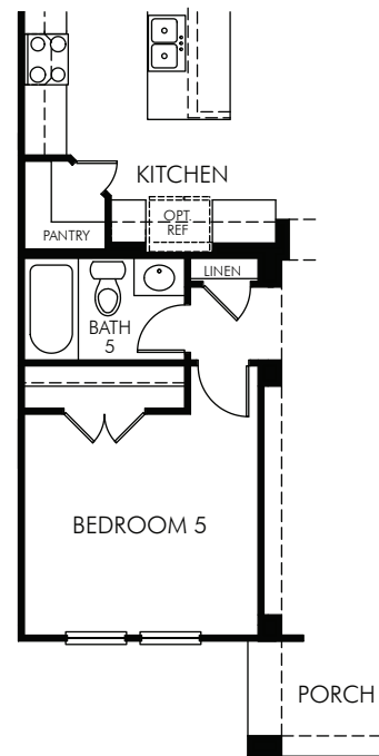
⑨ OPT. BEDROOM 5/BATH 5 BTH0505 WINDOW CONFIGURATIONS VARY BY ELEVATION
