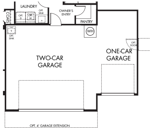
OPT. THREE-CAR GARAGE
