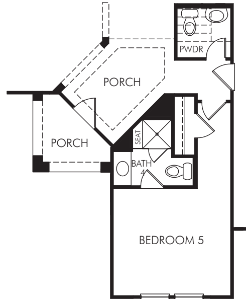
⑦ OPT. BEDROOM 5 / BATH 4 BED0503
