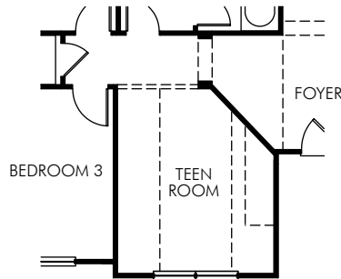
⑧ OPT. TEEN ROOM RMO0065
