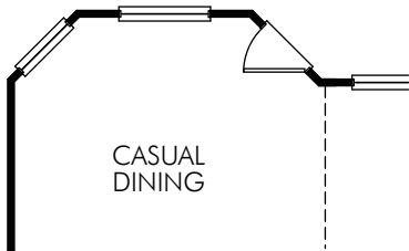
④ OPT. BAY AT CASUAL DINING -adding up to 40 sq ft. BAY0008
