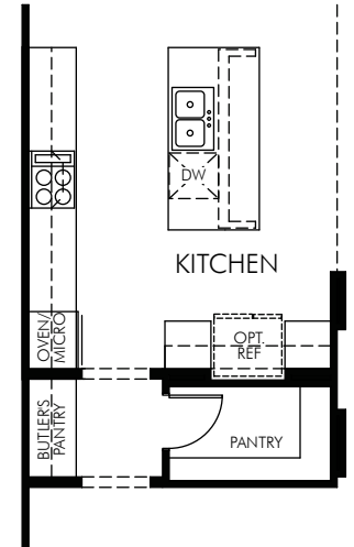
③ OPT. BUILT-IN KITCHEN KIT1002
