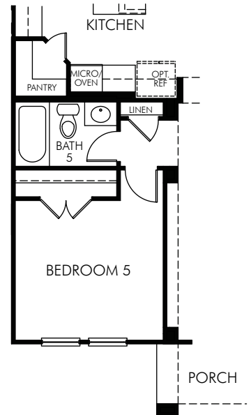
⑬ OPT. BEDROOM 5 /BATH 5 w/OPT. KITCHEN BTH0505/ KIT1000 WINDOW CONFIGURATIONS VARY BY ELEVATION
