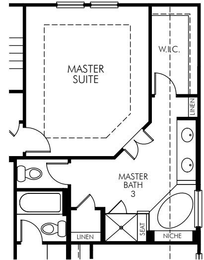
⑦ OPT. MASTER BATH 3 BTH0104
