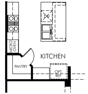
③ OPT. BUILT-IN KITCHEN KIT1000
