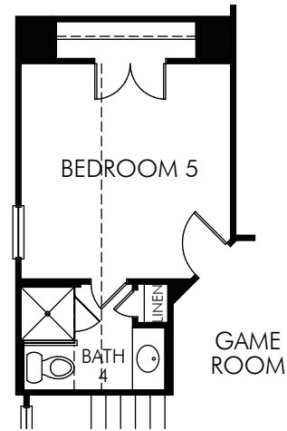
⑬ OPT. BEDROOM 5/BATH 4 -adding 49 sq. ft. BED0504
