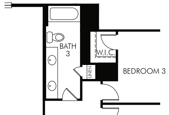
⑦ OPT. BATH 3 -adding 92 sq. ft. BTH0130
