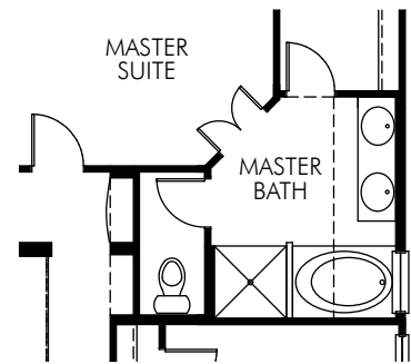
⑥ OPT. DELUXE MASTER BATH (BTH0115)
