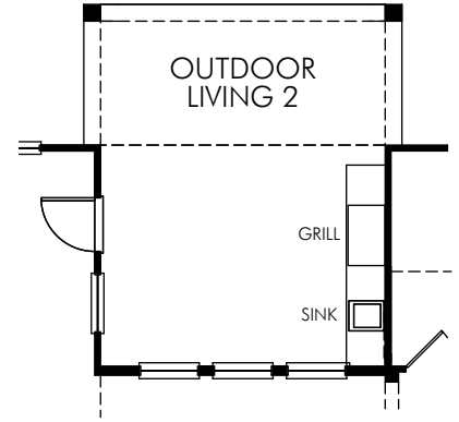
③ OPT. OUTDOOR LIVING 2 W/ KITCHEN KIT0002
