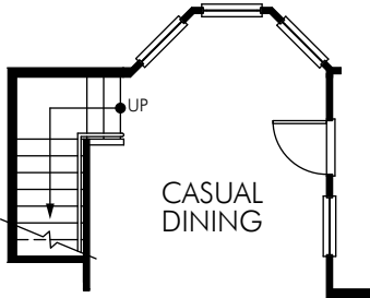
④ OPT. BAY AT CASUAL DINING BAY0002
