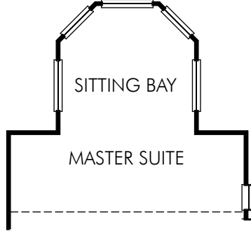
⑤ OPT. SITTING BAY AT MASTER SUITE RMO0023
