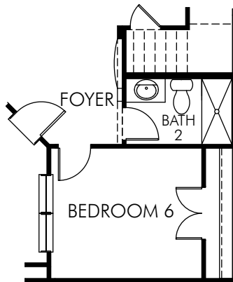
⑫ OPT. BEDROOM 6 W/BATH BED0604
