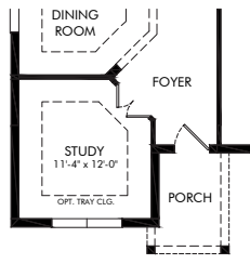
OPT. STUDY ILO LIVING ROOM
