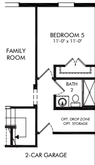
OPT. BEDROOM 5 WITH FULL BATH ILO FLEX
