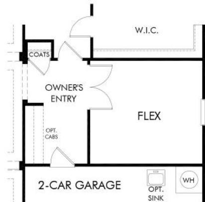
OPT. FLEX ILO BEDROOM 4
