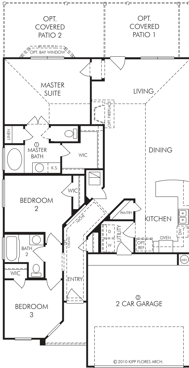
FIRST FLOOR
