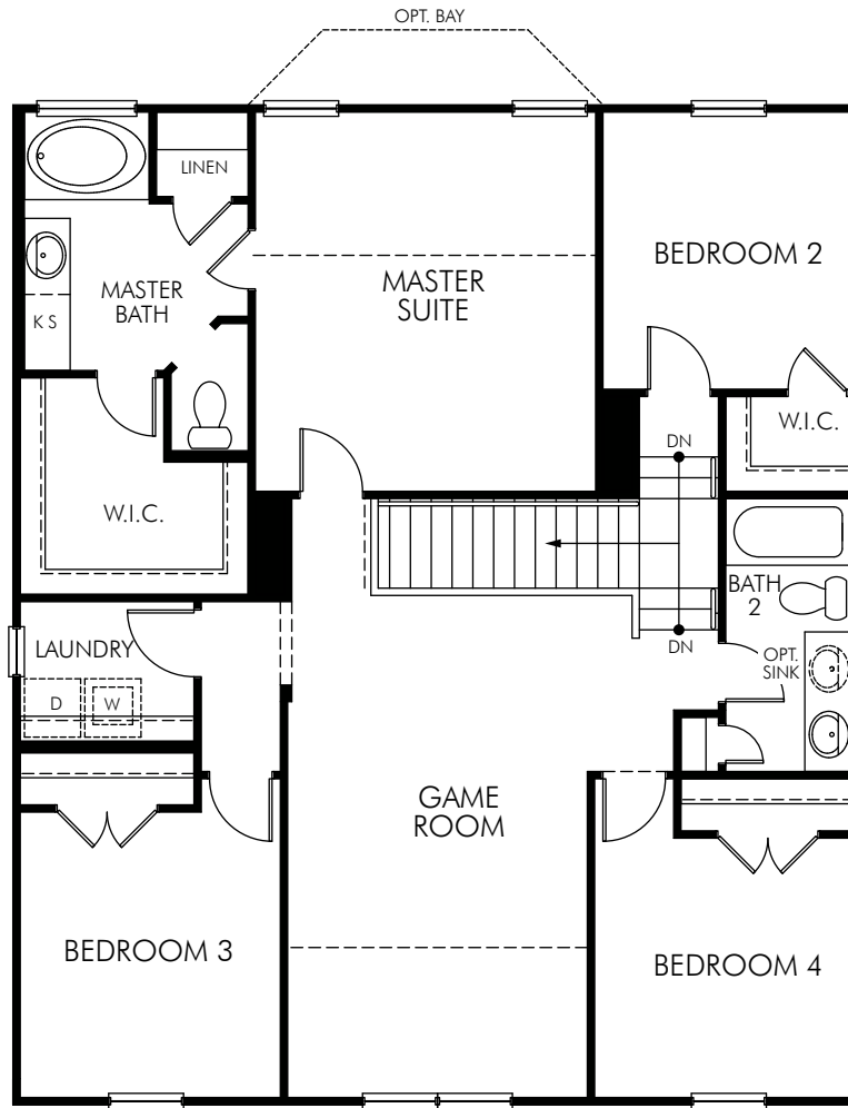
SECOND FLOOR
