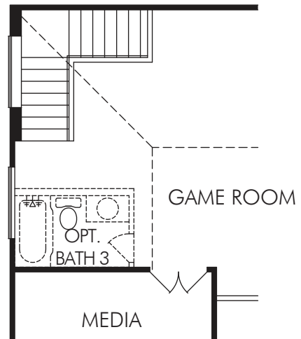
③ STAIRS W/ OPTIONAL 9'-1 1/8" 1ST FLOOR PLATE
