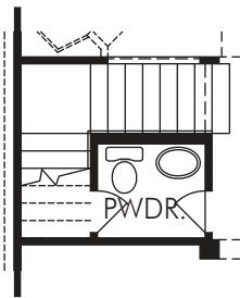
② STAIRS W/ OPTIONAL 9'-1 1/8" 1ST FLOOR PLATE
