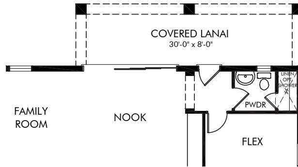
OPTIONAL COVERED LANAI 2
