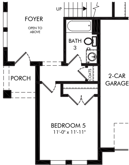
OPT. BEDROOM 5 WITH FULL BATH ILO STUDY
