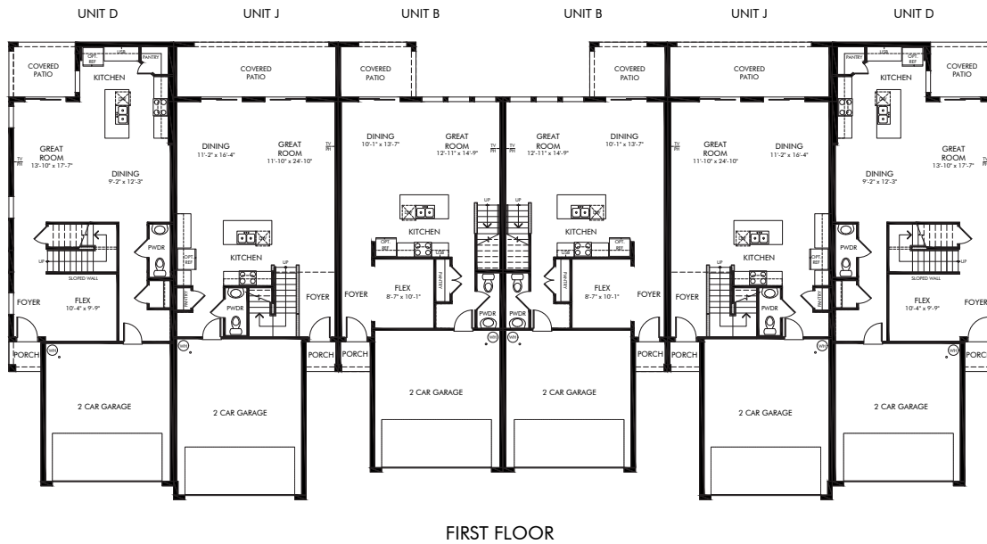
FIRST FLOOR
