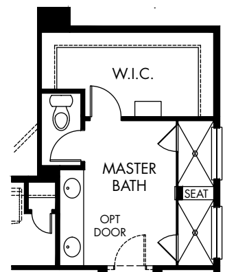
OPTIONAL DUAL SHOWER MASTER BATH LAYOUT
