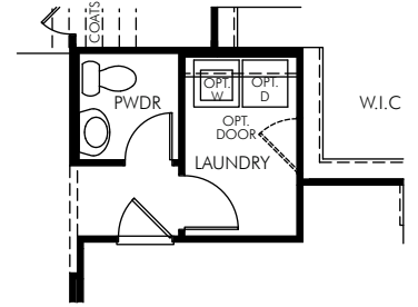
③ OPT. POWDER ROOM (BTH0303)
