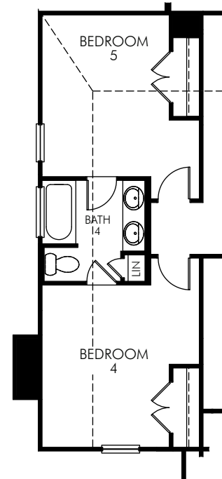
⑩ OPT. BATH 4 (BTH0140)
