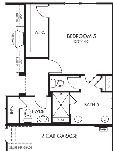
OPT. BEDROOM 5 & BATH 5
