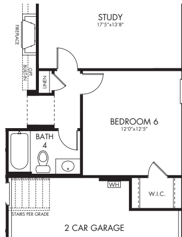
OPT. BEDROOM 6 & BATH 4
