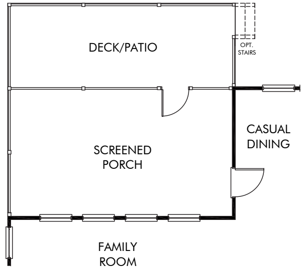
OPT. SCREENED PORCH WITH EXTENDED DECK/PATIO
