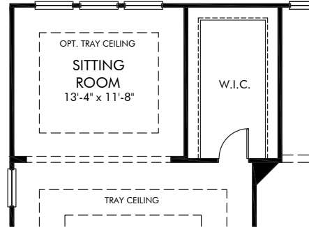
OPT. SITTING ROOM
