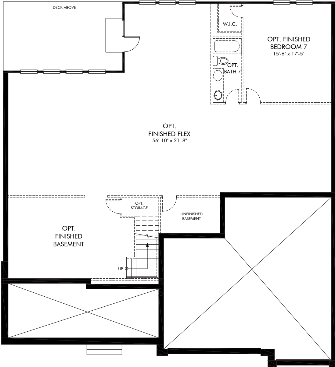
OPT. BASEMENT WITH OPTIONAL FLEX, BEDROOM 7, & BATH 7
