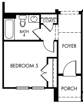
⑥ OPT. BEDROOM 5/ BATH 4 BED0503 WINDOW CONFIGURATIONS VARY BY ELEVATION
