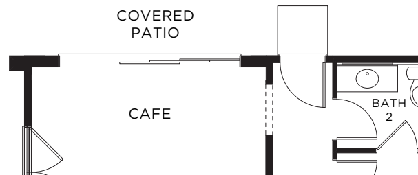
OPT. MULTI-SLIDE DOOR AT CAFE AT COVERED PATIO EXTENSION
