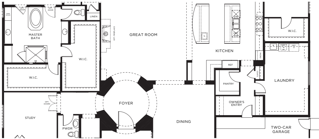
OPT. EXTENDED LAUNDRY ILO TANDEM AND EXTENDED MASTER W.I.C.
