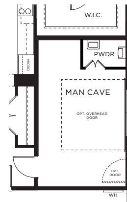
OPT. MAN CAVE WITH BATH
