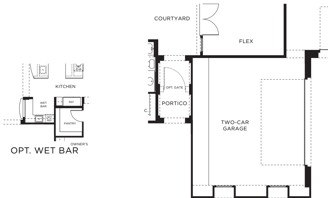
OPT. TWO-CAR GARAGE
