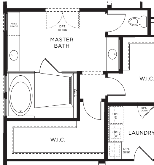
OPT. SPA MASTER BATH
