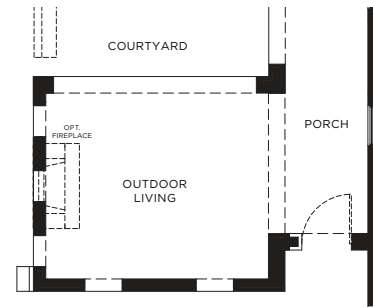
OPT. OUTDOOR LIVING ILO CASITA
