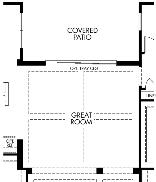
OPT. MULTI-SLIDE DOOR AT GREAT ROOM
