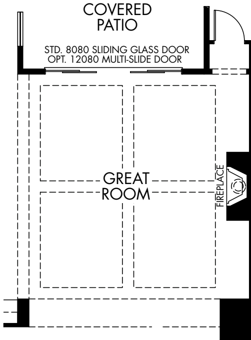
OPT. FIREPLACE AT GREAT ROOM
