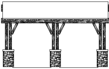
OPT. ELEVATION F CABANA FRONT
