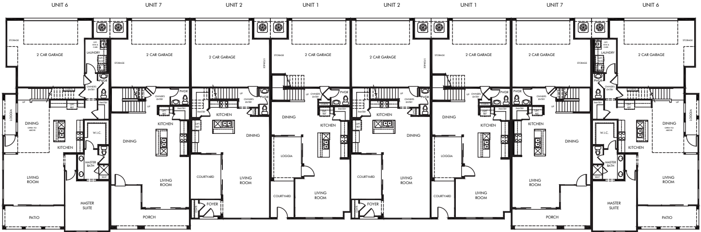
FIRST FLOOR
