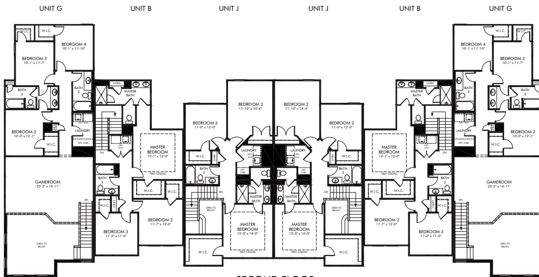
SECOND FLOOR
