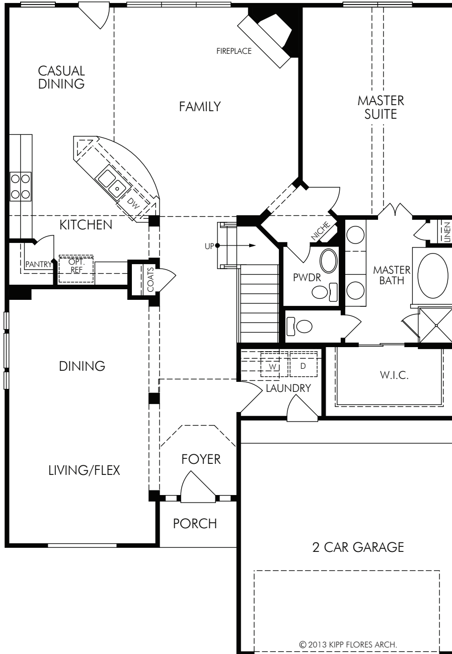
FIRST FLOOR
