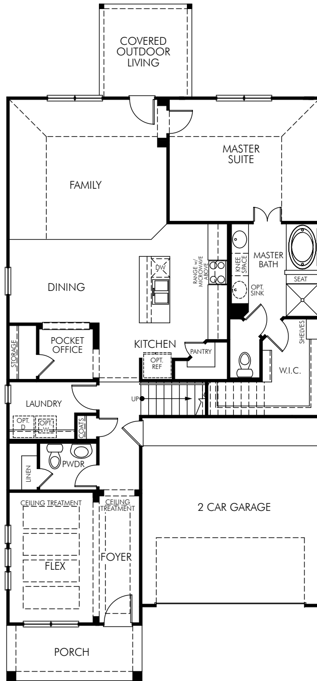
The Somerville | Plan 3L17 | First Floor 2,496 sq. ft. | 4 Bed | 2.5 Bath | 2 Car Garage | 2 Story
