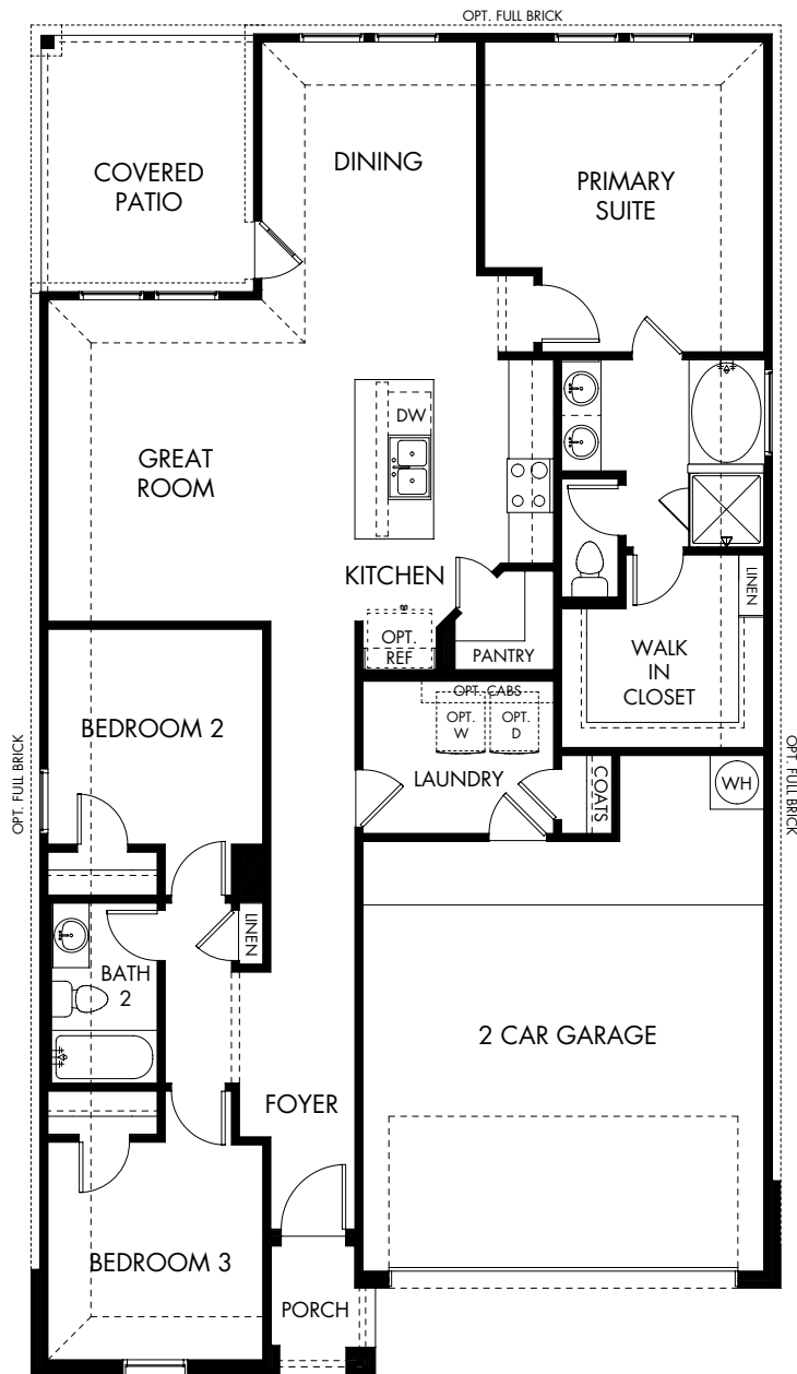
The Briscoe | Plan 820 | First Floor 1,477 sq. ft. | 3 Bed | 2 Bath | 2-Car Garage | 1 Story
