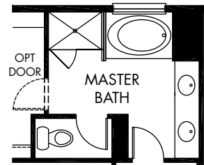
OPTIONAL FIVE-PIECE MASTER BATH LAYOUT
