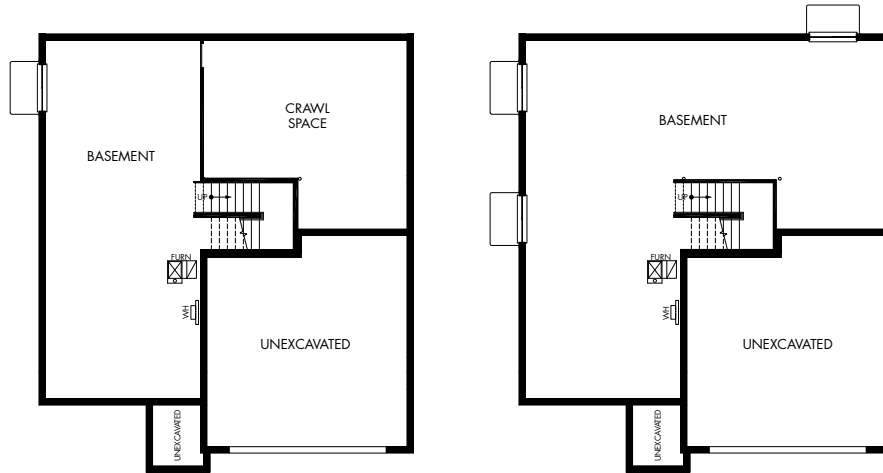
STANDARD BASEMENT
