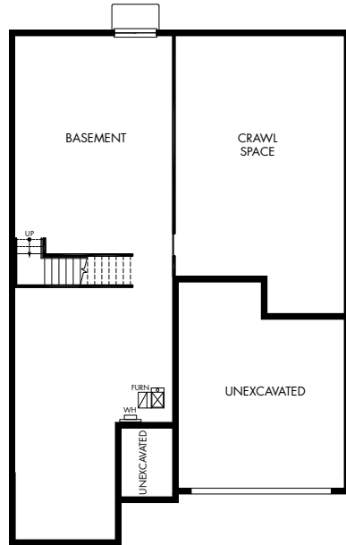
STANDARD BASEMENT
