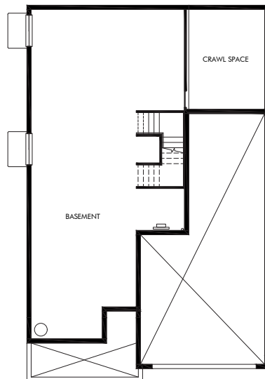
STANDARD BASEMENT
